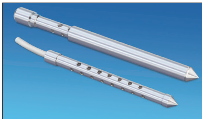
Model 615 Drive-Point and Shielded Drive-Point Piezometer
